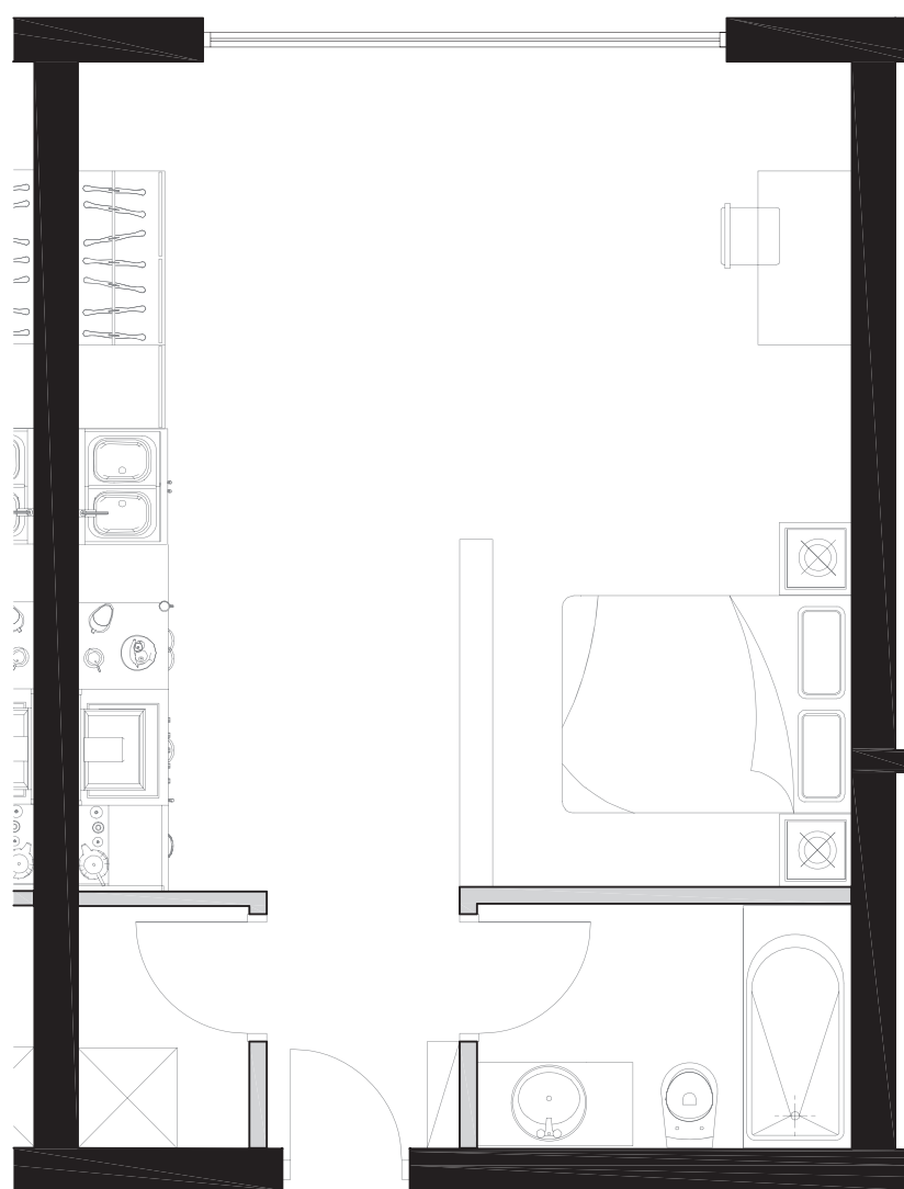
STUDIO LAYOUT
